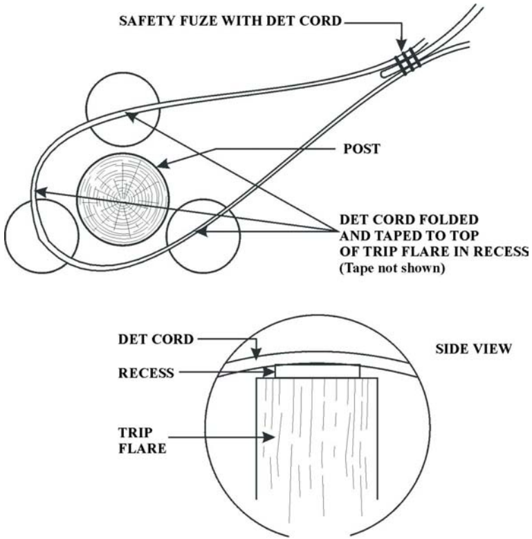
Figure C-2: Initiation of Trip Flare—Detonating Cord Taped to Top of Flare Recess
