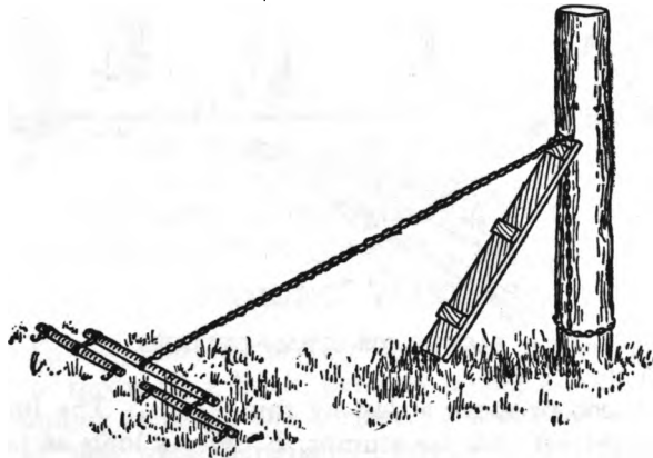
POST PULLER IN POSITION
