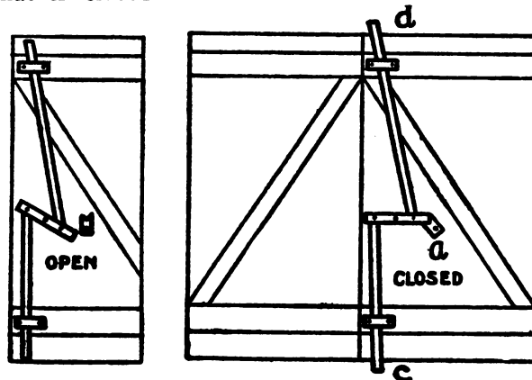
LATCH FOR DOUBLE DOORS
