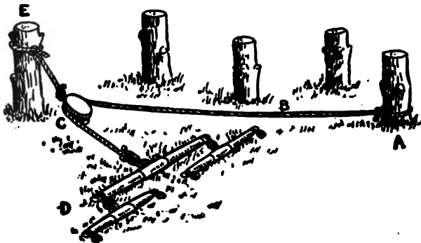
TACKLE FOR STUMP-PULLING
