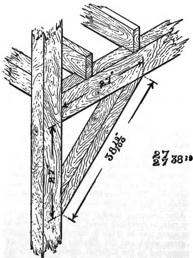
BRACE RULE
