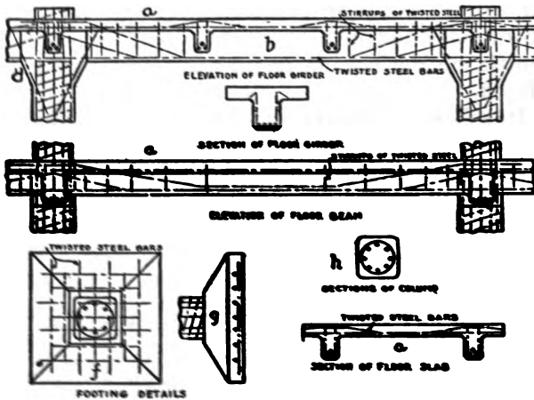
DETAILS OF REINFORCEMENT
