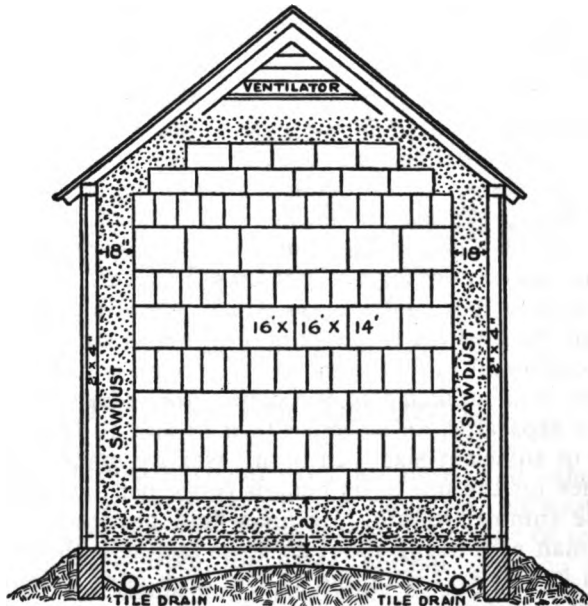
CROSS-SECTION OF ICEHOUSE
