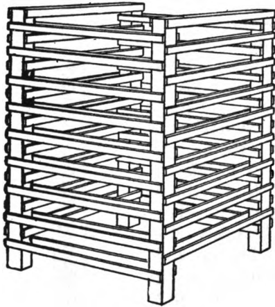
CORN DRYING RACK
