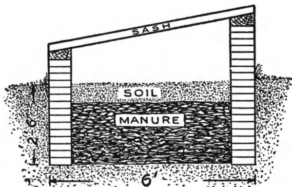
HOTBED WITH BRICK WALLS
