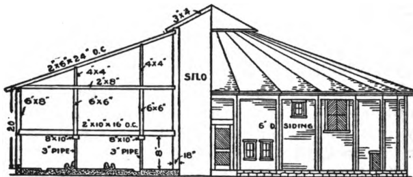
CROSS-SECTION OF BARN
