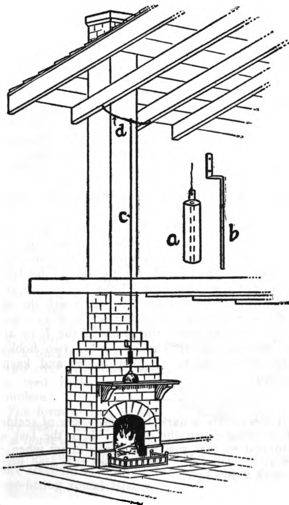
A FIRE ALARM
