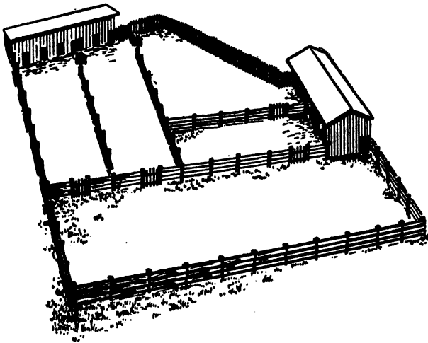
FIG HOUSES AND PENS
