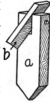
GATE CATCH
