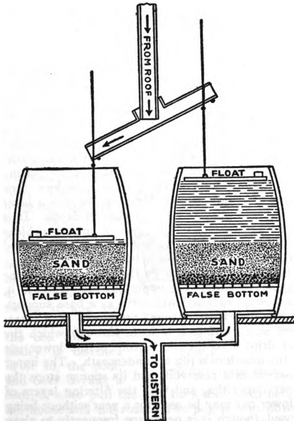
TWO-BARREL FILTER
