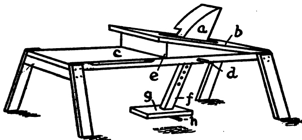
SHAVING HORSE
