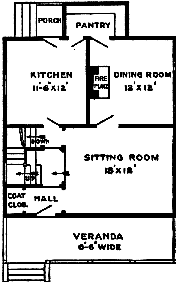
FIRST FLOOR COTTAGE PLAN
