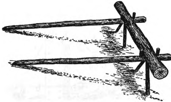
FIGURE 2—SKIDWAY
