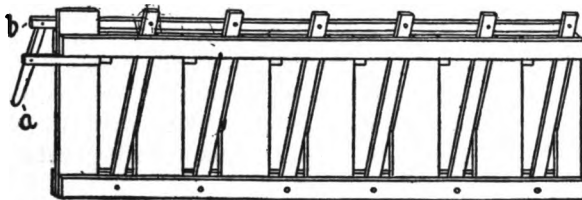
STANCHIONS FOR CALVES
