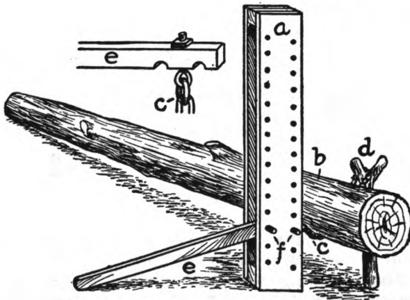
FIGURE 4—LOG JACK
