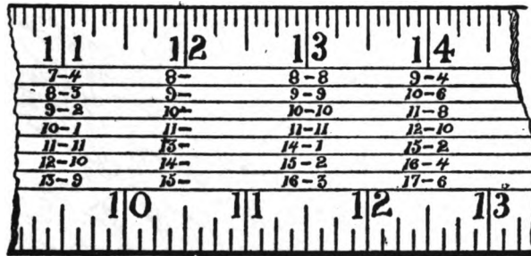
LUMBER RULE
