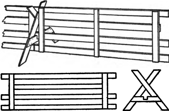
MOVABLE FENCE AND PARTS
