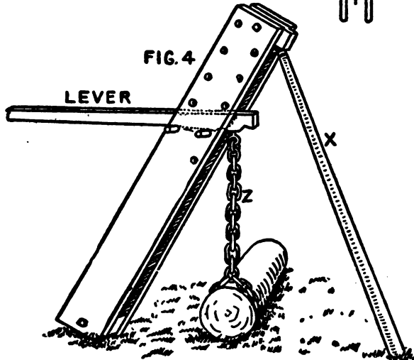
WEIGHT LIFTER AND DETAILS
