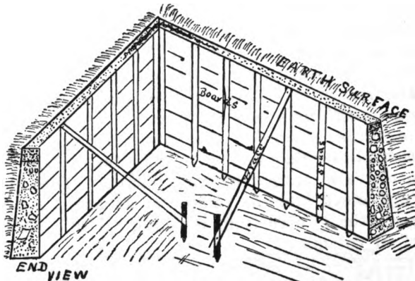
CONCRETE CELLAR WALL
