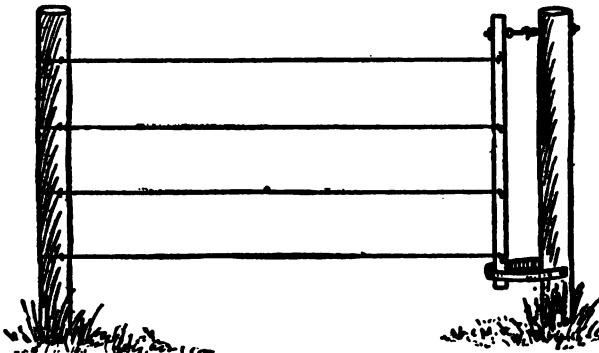
WIRE GATE THAT SPEAKS FOR ITSELF
