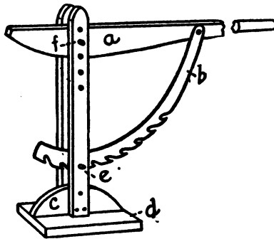
WAGON JACK
