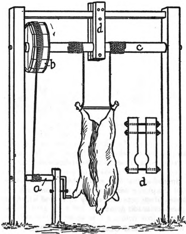
CARCASS DERRICK
