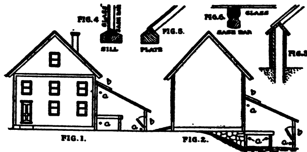
DETAILS FOR SMALL GREENHOUSES
