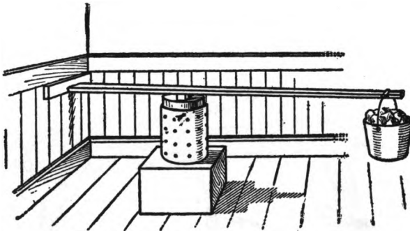
CHEESE PRESS
