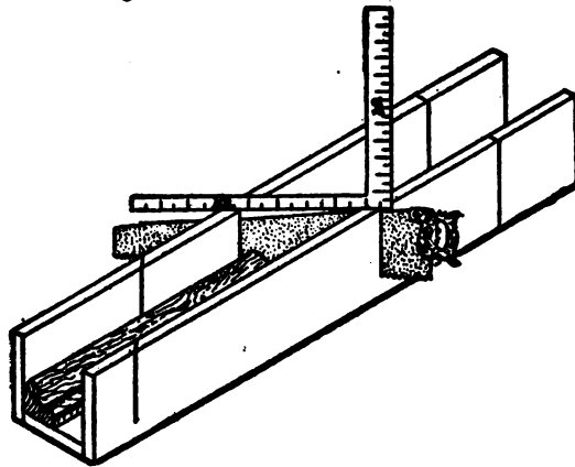
FIGURES 2 AND 3
