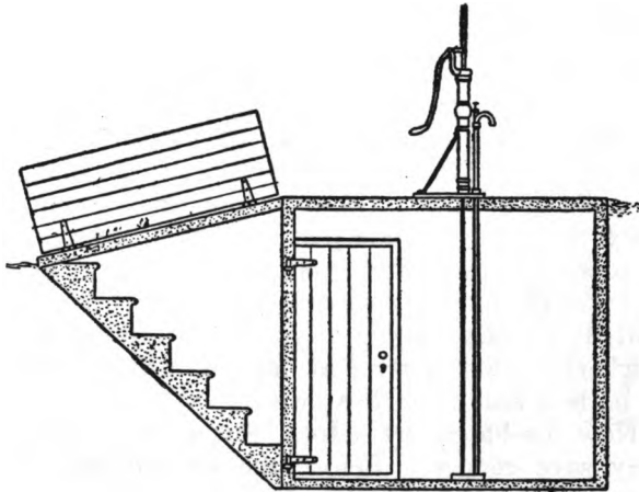
CONCRETE OUTDOOR CELLAR
